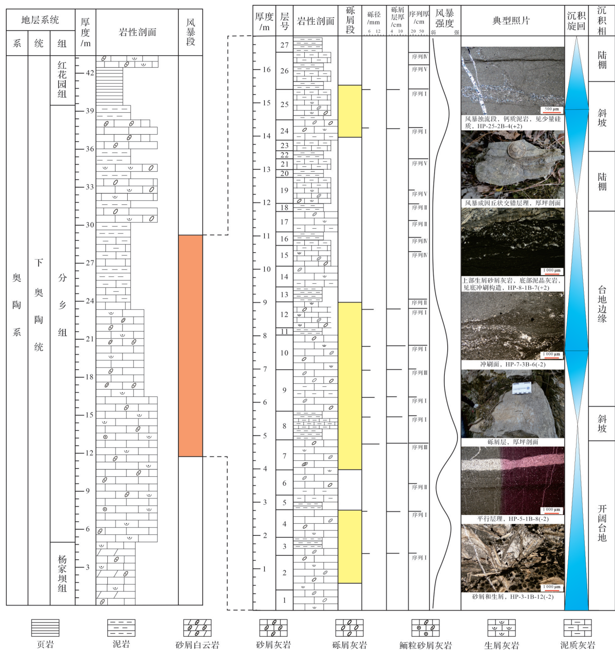
图2 城口地区厚坪剖面下奥陶统分乡组风暴沉积综合柱状图 Fig.2 Comprehensive histogram of storm deposition of the Lower Ordovician Fenxiang Formation in the Houping section, Chengkou area
