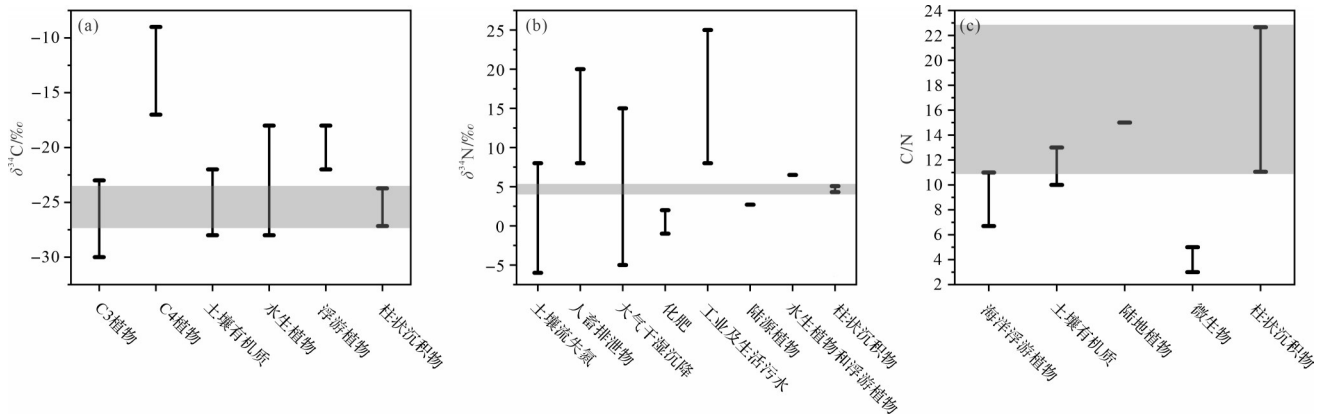
图6 柱状沉积物中 \delta^{13}\text{C} 、 \delta^{15}\text{N} 和C/N的来源分布特征 Fig.6 Source distribution of \delta^{13}\text{C} , \delta^{15}\text{N} and C/N in columnar sediments
