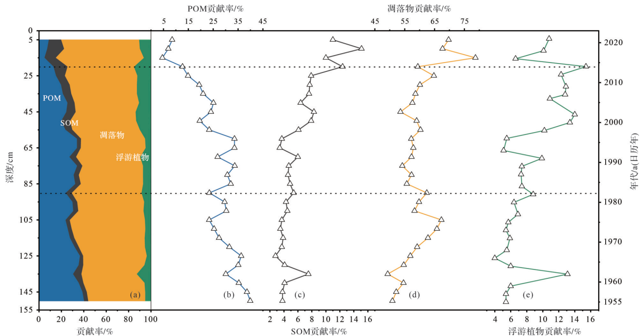
图7 柱状沉积物中有机碳潜在来源贡献率及其分布特征 Fig.7 Contribution rate and distribution of potential sources of TOC in columnar sediments
