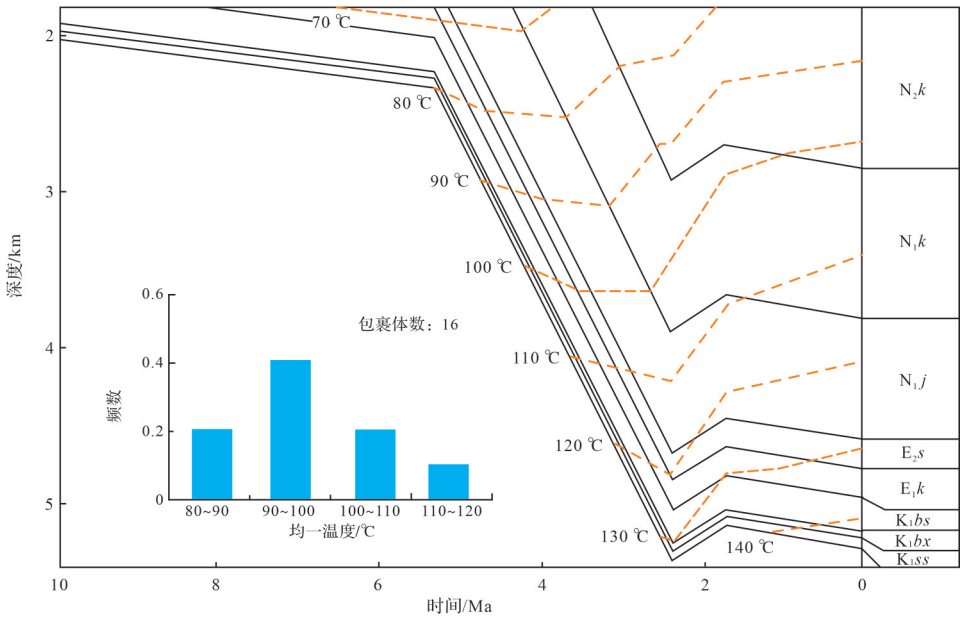
图 13 英买 467 井盐水包裹体均一温度和埋藏史 (据文献[29]修改) Fig.13 Homogenization temperature and burial history of brine inclusions in well Yingmai 467 (modified from reference [29])
