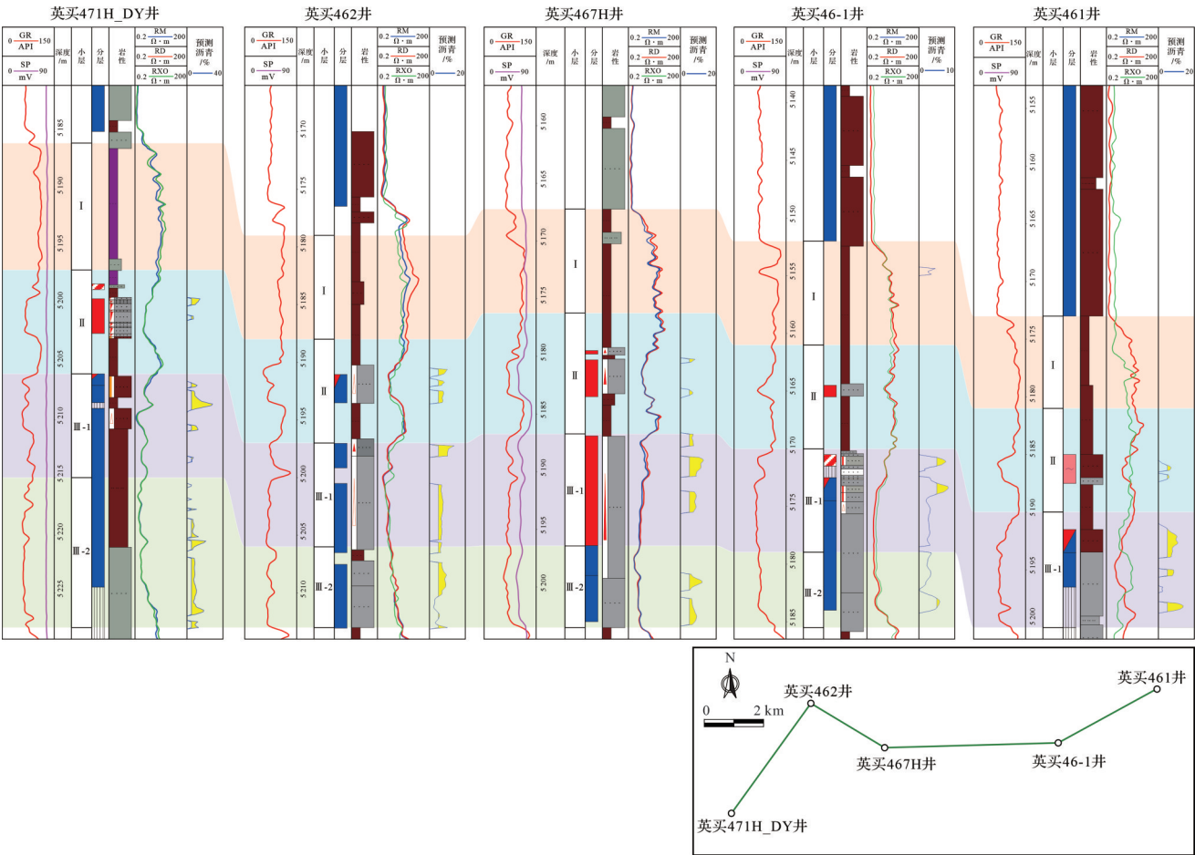
图 12 英买 471H 井—英买 462 井—英买 467H 井—英买 46-1 井—英买 461 井白垩系巴西改组沥青含量连井剖面图 Fig.12 Well Yingmai 471H-well Yingmai 462-well Yingmai 467H-well Yingmai 46-1-well Yingmai 461 Cretaceous Baxigai Formation bitumen content well profiles
