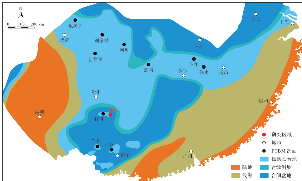
图1 华南早三叠纪古地理图,显示田湾剖面的古地理背景(底图据冯增昭等, 1997 修改) Fig.1 Early Triassic paleogeographical map of South China showing the setting of the Tianwan section (base map modified from Feng et al. , 1997)
