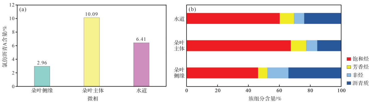
图 14 庆城地区长 7_{1-2} 亚段不同微相砂岩氯仿沥青“A”(a)及族组分含量(b)分布图 Fig. 14 Distribution of chloroform bitumen “A” (a) and group component content (b) for different microfacies sandstones in Chang 7_{1-2} sub-member, Qingcheng area
