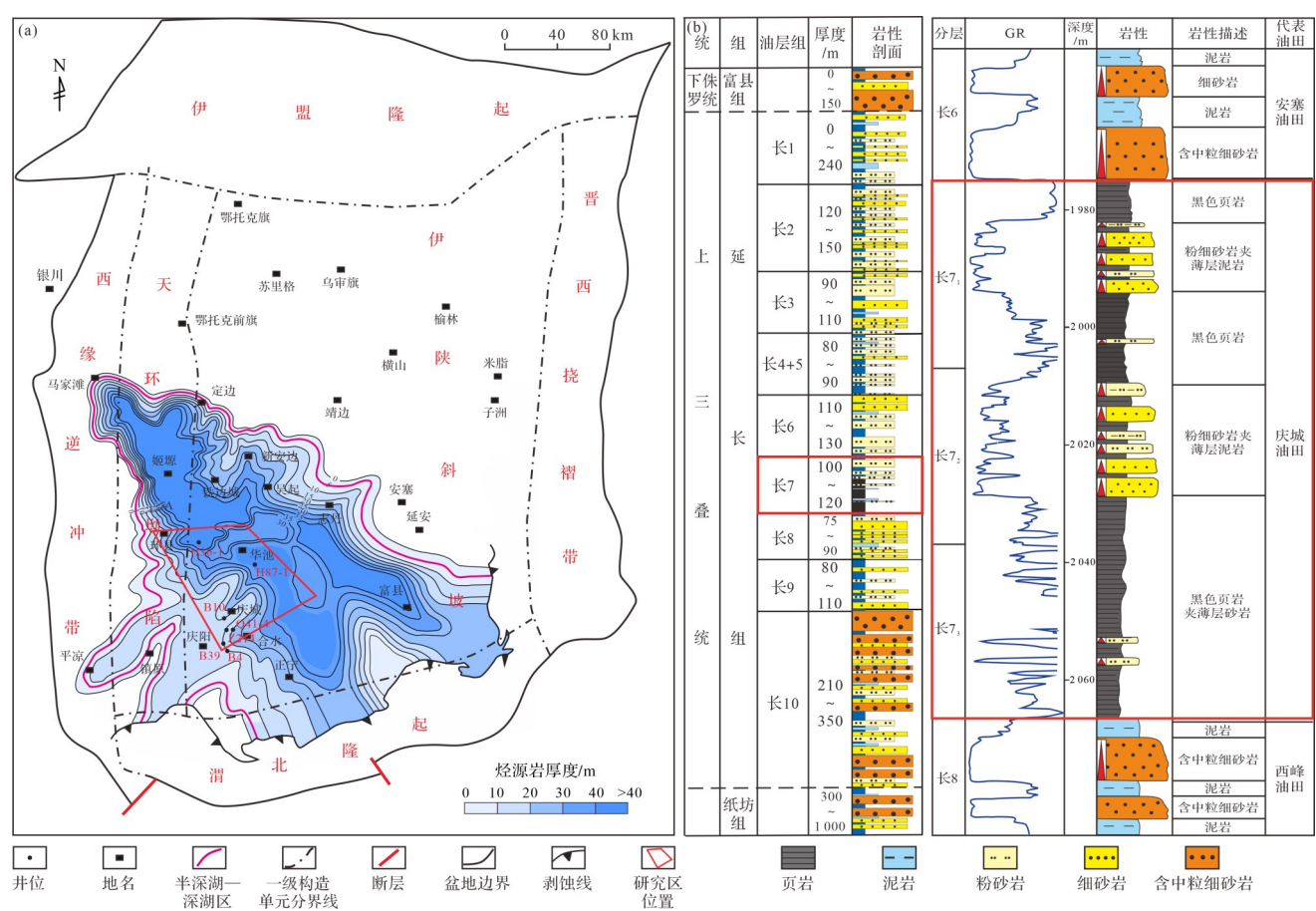
图1 鄂尔多斯盆地长7沉积期烃源岩分布(a)与延长组地层特征(b) Fig. 1 Distribution of source rocks (a) and stratigraphy (b) of the Yanchang Formation in the Chang 7 sedimentary period, Ordos Basin
