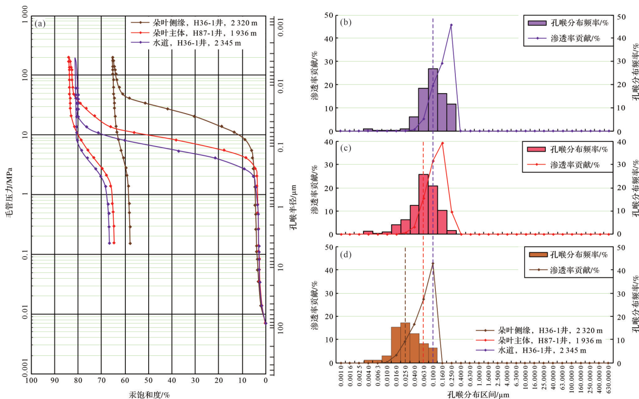
图 10 庆城地区长 7_{1-2} 亚段不同微相砂岩高压压汞典型曲线 (a) 及孔喉分布特征 (b-d) Fig. 10 Typical curves of high-pressure mercury intrusion (a) and pore throat distribution (b-d) properties of different microfacies sandstones in Chang 7_{1-2} sub-member, Qingcheng area
