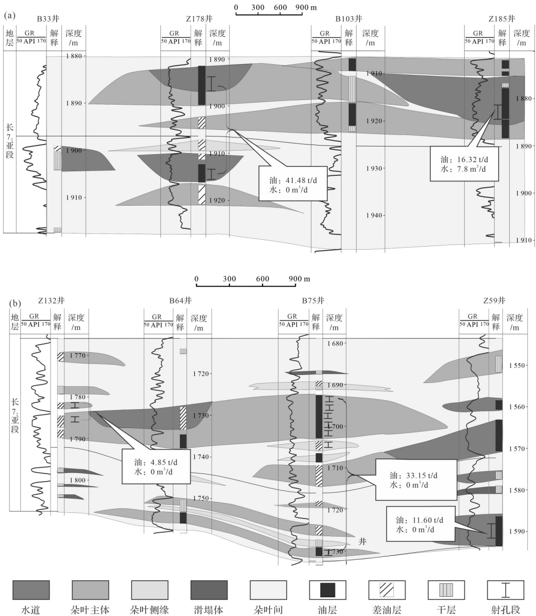
图 15 庆城地区长 7_{1-2} 亚段不同微相砂岩试油结果 (a)B33井—Z185井沉积微相剖面图;(b)Z132井—Z59井沉积微相剖面图 Fig. 15 Oil test results of sandstones with different microfacies in Chang 7_{1-2} sub-member, Qingcheng area
