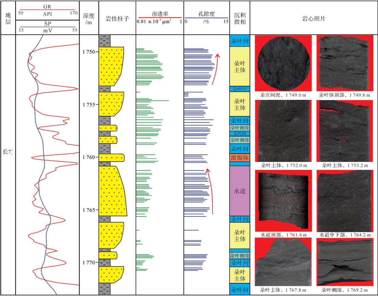
图4 庆城地区B4井长7 2 小层综合柱状图 Fig. 4 Comprehensive histogram of Chang 7 2 sublayer in well B4, Qingcheng area
