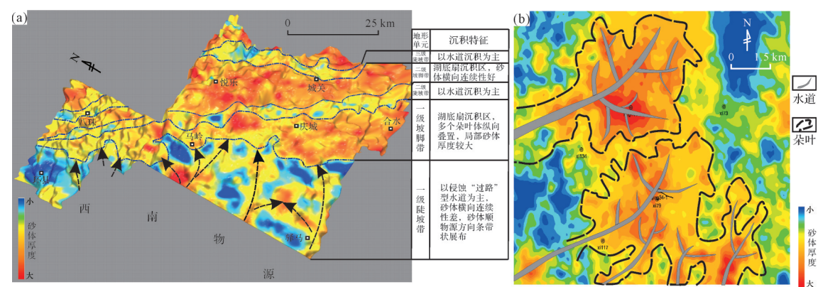
图2 鄂尔多斯盆地庆城油田长7段沉积古地形及湖底扇展布特征 (a)长7段湖底扇;(b)长7段湖底扇局部地震切片(图a红色框) Fig. 2 Sedimentary paleotopography and sublacustrine fan distribution of the Chang 7 member in Qingcheng oilfield, Ordos Basin
