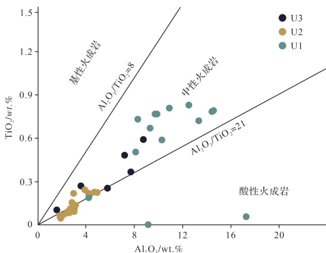
图6 \text{TiO}_2 - \text{Al}_2\text{O}_3 物源判别图解 (Hayashi et al. , 1997)
